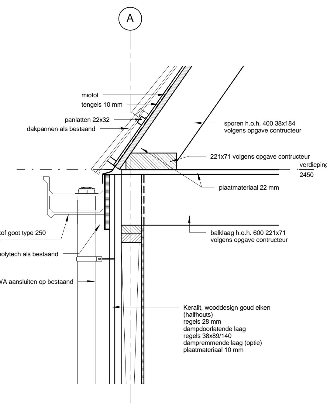
principe detail 2.
