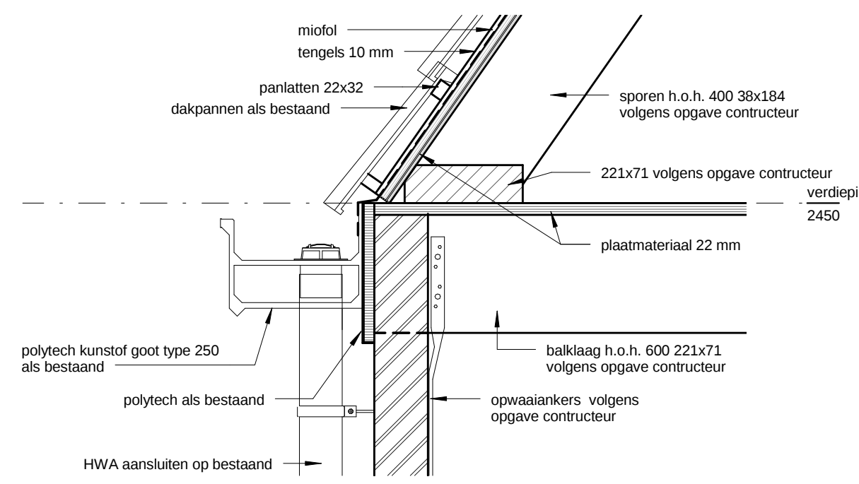
principe detail 2.
